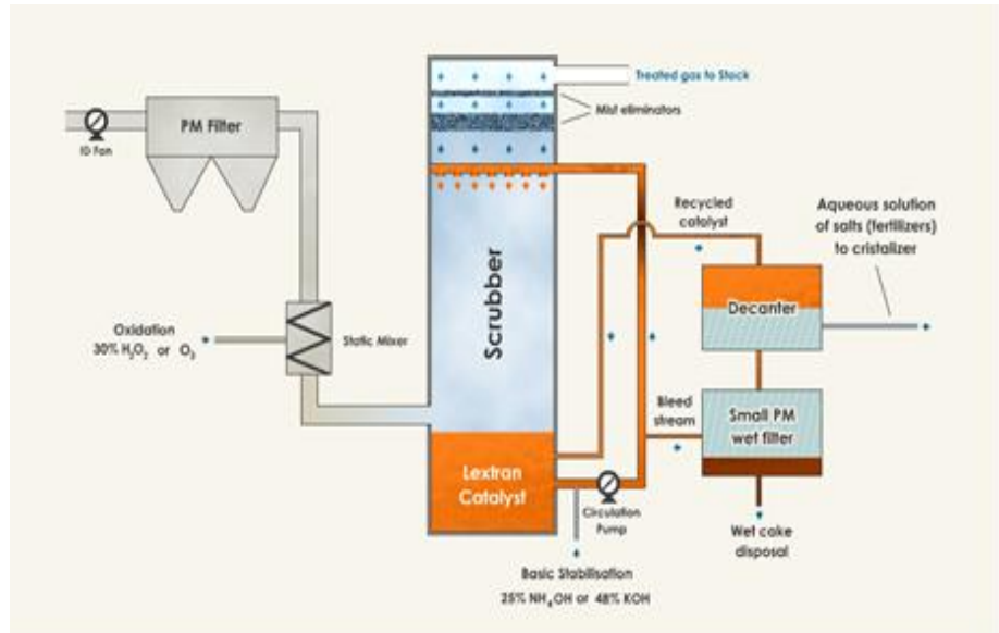
Figure 2. Schematic design of Lextran's WFGD-based operation. Removes NO x and SO x from flue gas and converts them into fertilizers. Heavy metals form a stable complex with Lextran makeup not interfering with the De-SO x and De-NO x process.
